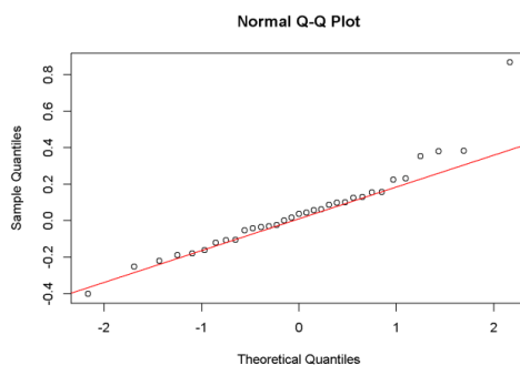
Gambar 4.6 Plot Normal Q-Q
