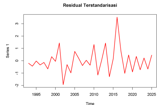
Gambar 4.4 Plot Residual Terstandarisasi
