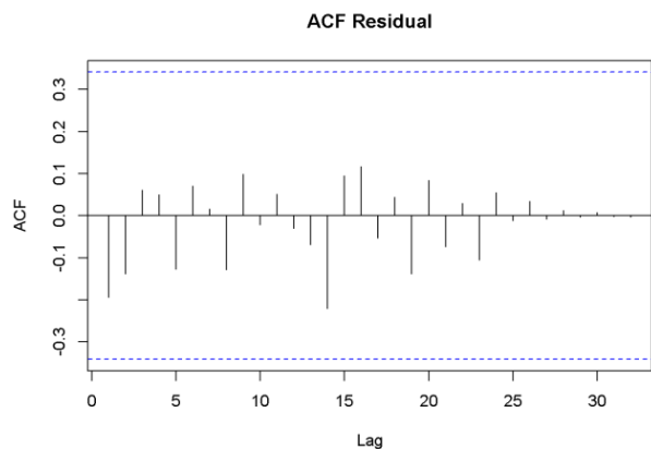
Gambar 4.5 Plot ACF Residual
